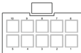
Viewed from Wire side of Plug Deluxe Version Pin Out
