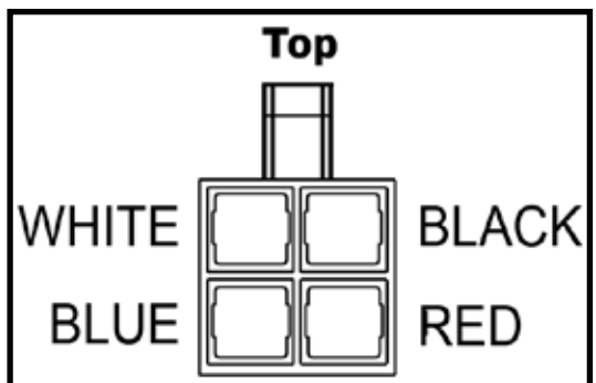
Diagram above shows back of plug (larger end). This is the end to plug the terminals into.
